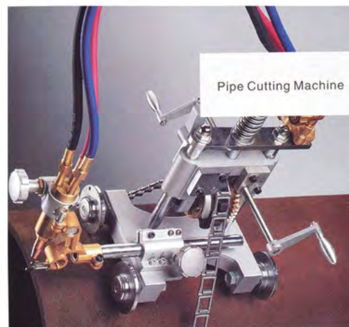
J-1011 CUTTING MACHINE
